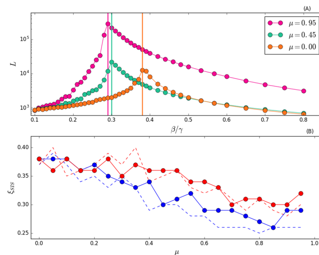
Figure 5. Panel (A) Lifetime of the disease L as a function of \beta/\gamma , for selected values of \mu and when s_{\min} = 10 . Vertical lines are the epidemic threshold. Panel (B) Ratio \xi_{SIS} = \beta/\gamma in correspondence of L_{\max} as a function of \mu . In red curves we set s_{\min} = 100 , blue curves s_{\min} = 10 . Each point is an average of 10^2 independent simulations. Note that we avoid to simulate \mu = 1 because the criterion we follow for the estimation of the threshold does not hold for a network with many connected components.
