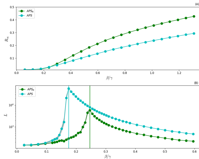
Figure 6. Panel (A) R_{\infty} as a function of \beta/\gamma for SIR processes diffusing on APS (cyan circles) and on the randomized APS dataset (green circles). Panel (B) L as a function of \beta/\gamma for a SIS models evolving on the same two networks. Each point is the average of 10^2 independent simulations started from 1% of random seeds. We fix \gamma = 0.05 .
