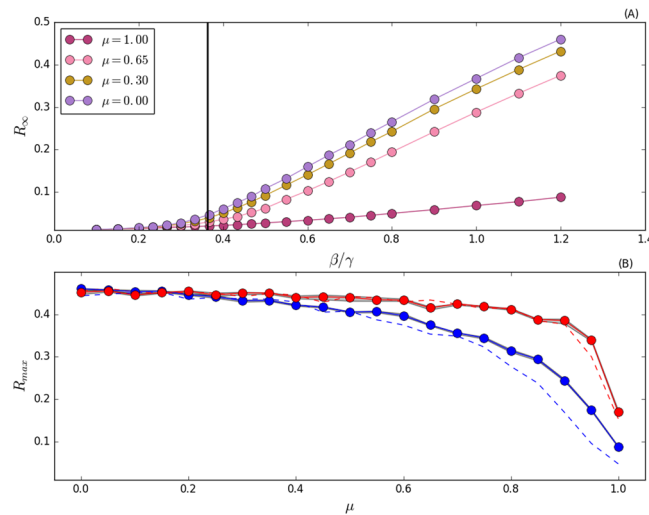
Figure 4. Panel (A) R_{\infty} as a function of \beta/\gamma , for selected values of \mu and s_{\min} = 10 . Vertical black line represents the theoretical value of the epidemic threshold for \mu = 0 as derived in refs 24,71 . Panel (B) R_{\max} , i.e. the max value of R_{\infty} , as a function of \mu . In red curves we set s_{\min} = 100 , in blue curves s_{\min} = 10 . In solid curves, we draw community sizes directly from the community size distribution P(s) . In dashed curves, we fix the community sizes as equal to the average value of P(s) for all communities. The 95% confidence interval is in grey. Each point is an average of 10^2 independent simulations.
