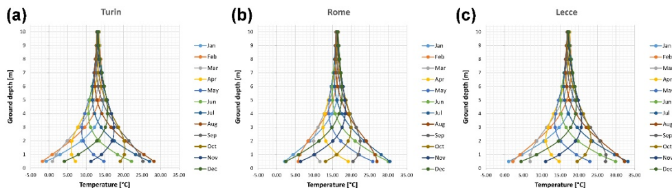
Fig. 1. Calculated ground temperature profiles considering different depths for (a) Turin; (b) Rome; (c) Lecce.
