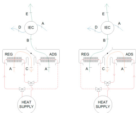
Figure 3 Scheme with two parallel dehumidifier (current)
