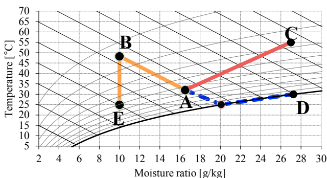
Figure 4. Air transformation on the psychrometric with isenthalpic adsorption (current)
