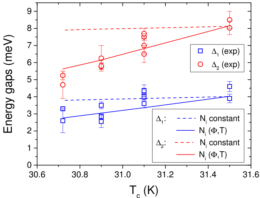
Figure 7. (Color online) Symbols: the experimental low temperature energy gaps of film N.316 (symbols) as a function of the critical temperature T_c^{90} . Lines: the same quantities calculated by numerical solutions of Eliashberg equations: in the standard case, i.e. with temperature-independent density of states at the Fermi level N_i (dashed lines) and by using temperature-dependent densities of states N_i(\Phi, T) (solid lines).
