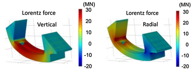
Fig. 9. Induced Lorentz forces in the divertor cassette shell plate (left: vertical, right: radial component).
