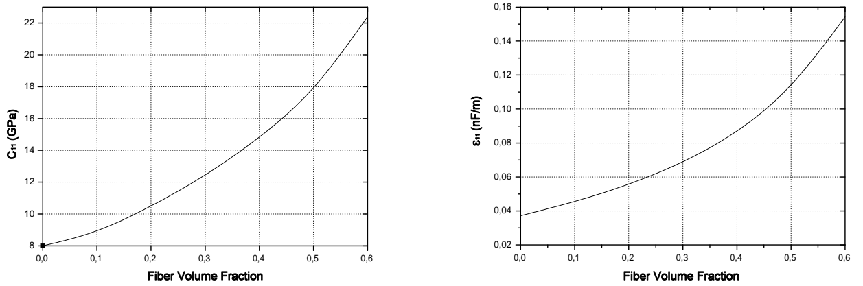
Figure 4. Effective properties versus PZT Fiber Volume Fraction HEX-RVE.
