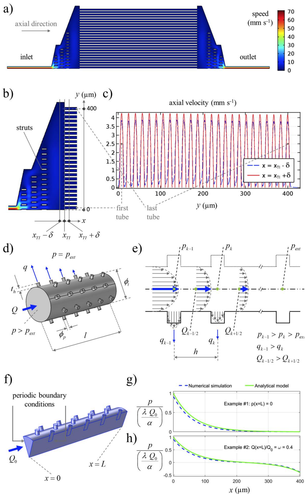
Figure 2. Modeling of the microfluidic system. a) Intensity plot of the fluid speed numerically computed on a simplified 2D geometry (half domain, by symmetry). b) Detail showing the struts supporting the junctions, and the considered cut-sections ( \delta = 0.01 \mu\text{m} ). c)
