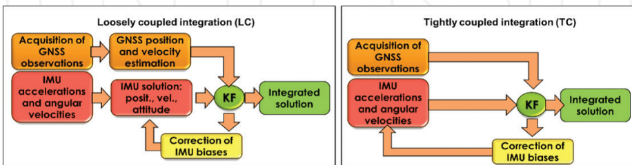
Figure 5. GNSS + INS processing approaches.
