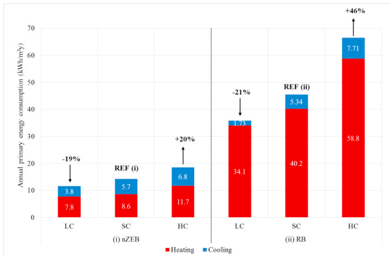
Fig. 5. Annual primary energy consumptions for space heating and cooling.
