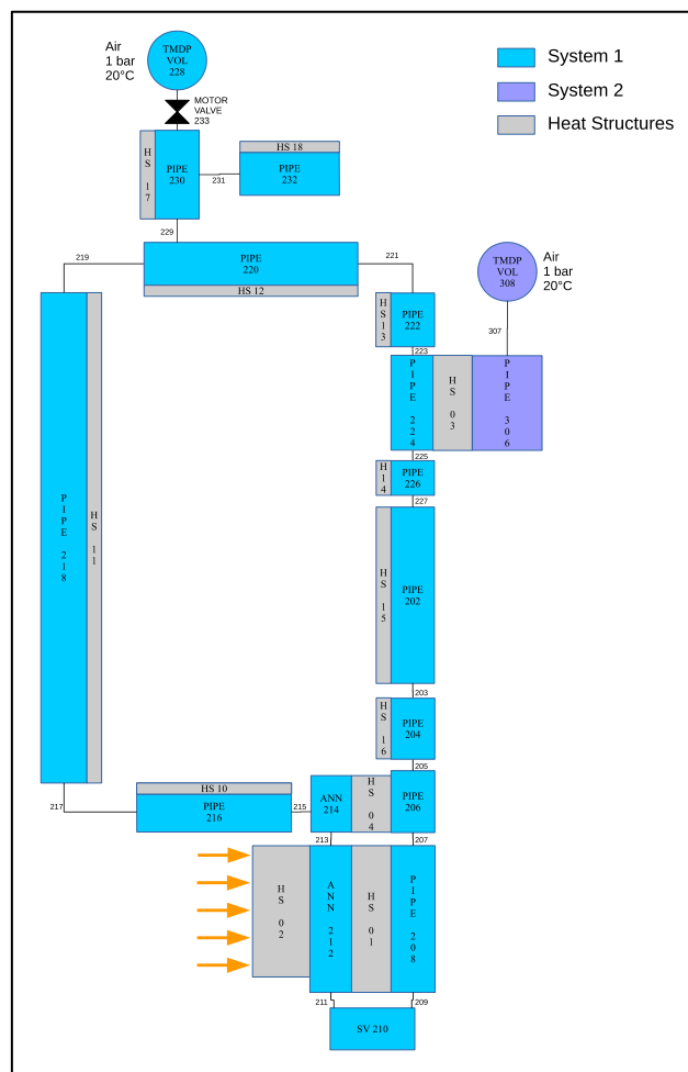
Figure 2: RELAP5-3D nodalization of the facility
