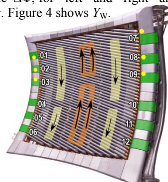
Fig. 1. 3-strap antenna with strap RF currents and measurement locations highlighted.
