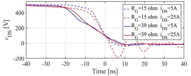
Fig. 17. Module #2 turn-on, behavior of V_{DS} for different values of gate resistor.
