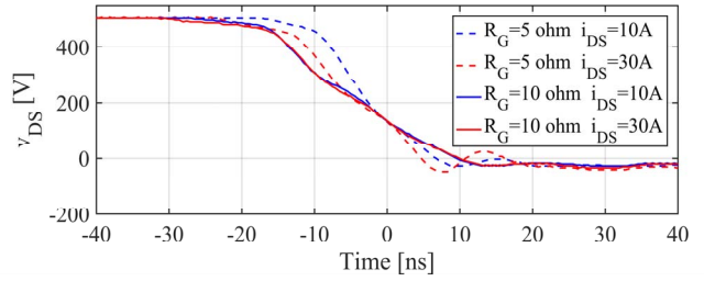
Fig. 16. Module #1 turn-on, behavior of V_{DS} for different values of gate resistor.
