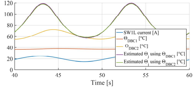
Fig. 23. Junction temperature estimation with sinusoidal current reference (module #2)
