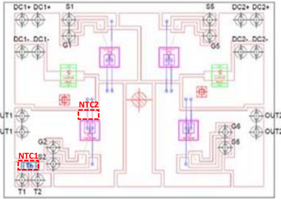
Fig. 2. Layout of power module (courtesy of Vishay Semiconductor Italiana). In green the two internal local capacitors. In blue the internal NTC resistor (label “Th”), for measurement of case temperature.
