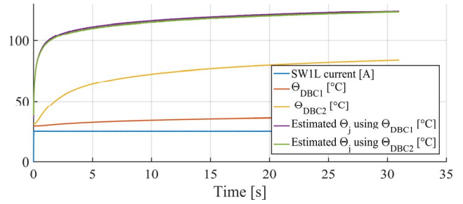
Fig. 22. Junction temperature estimation during a current step of 25 A (module #2)
