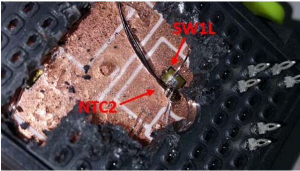
Fig. 21. Local NTC resistor label as “NTC2” in Fig. 2 positioned near the SWIL.
