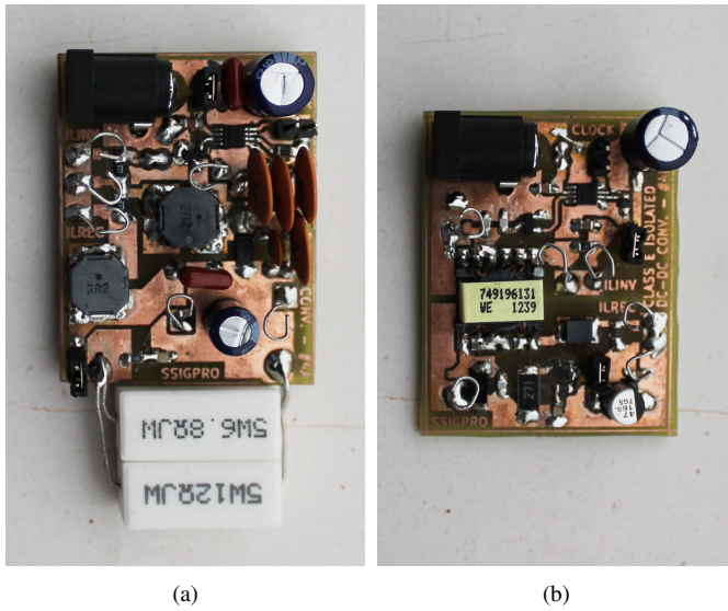
Fig. 9. Photograph of the designed prototypes. (a): 2.5 W non-isolated dc-dc converter; and (b): 500 mW isolated dc-dc converter.
