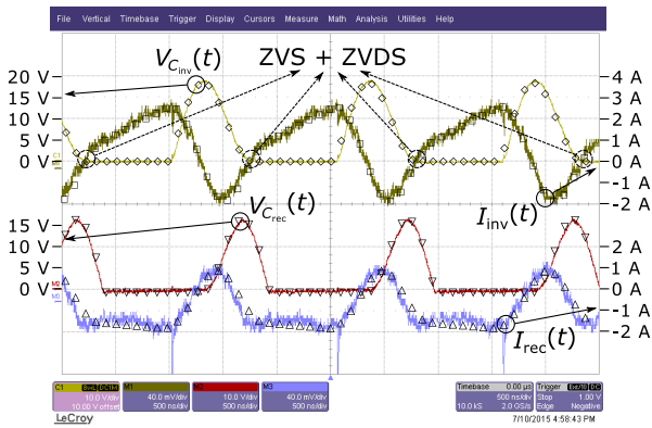
Fig. 10. Measured current and voltage waveforms for the 2.5 W non-isolated dc-dc converter prototype, compared with the expected theoretical ones (dark markers) computed with the proposed model.
