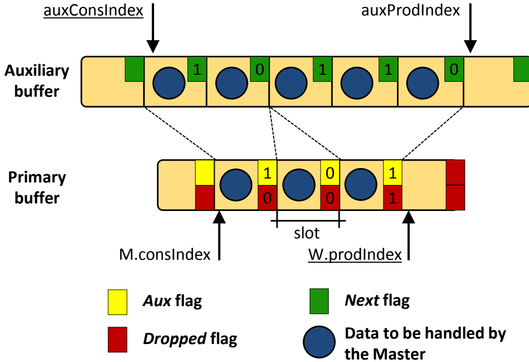
Figure 4: Binding primary buffer - auxiliary buffer.
