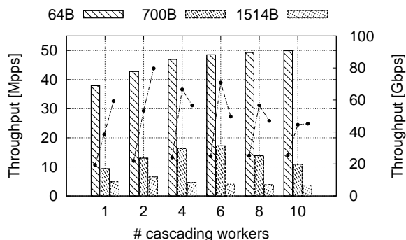
Figure 7: Internal throughput of the function chain, with real Workers and a 1M packets in memory.
