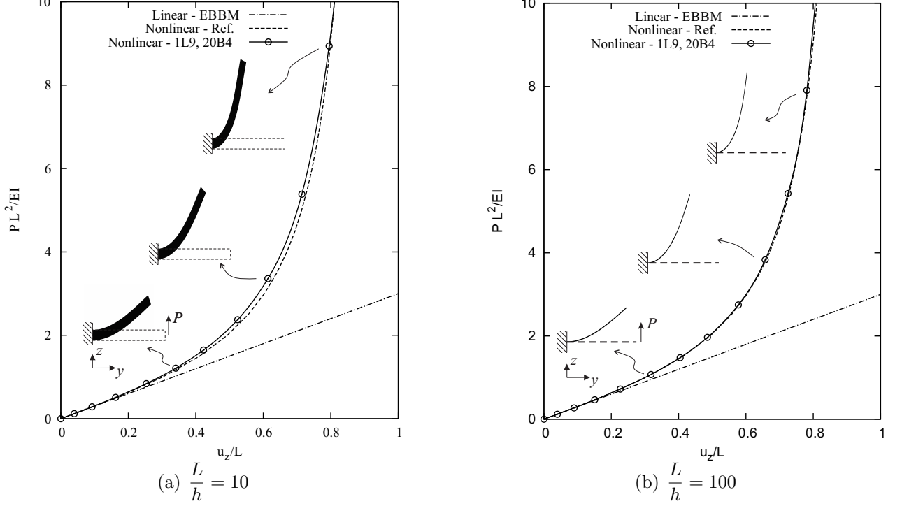
Figure 3: Equilibrium curves of the square cross-section beam subjected to vertical loading. Reference solution from [5].
