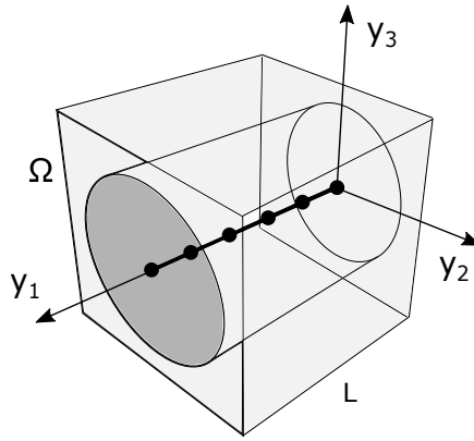
Figure 2. Reference system for the beam modeling of the UC.
