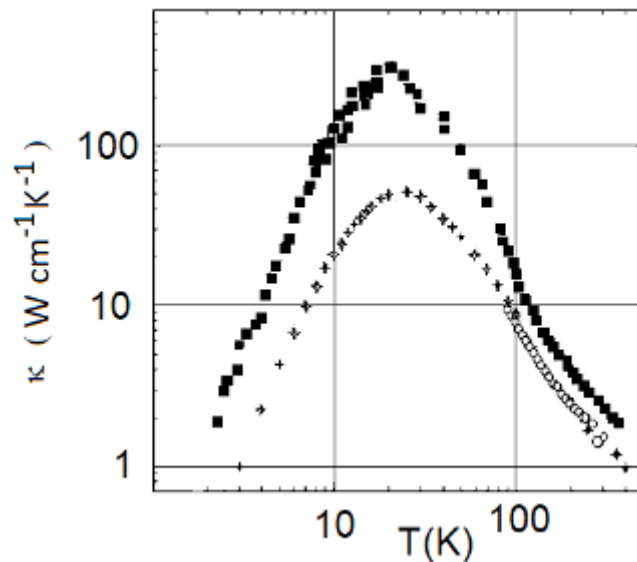
Fig. 4: Thermal conductivity of isotopically pure ^{28}\text{Si} and Si of natural isotopic abundance. Some data from Ref.26. The open dots represent the measurements on sample SIN1 of natural silicon. As told in [26] the “plus” symbols denote the “standard” curve for natural Si, as given by [27].
