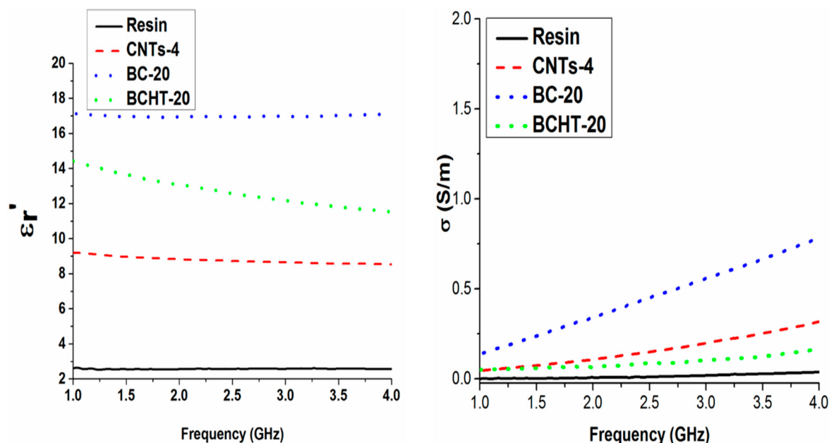
Figure 11. Comparison among the real part of permittivity ( left panel ) and conductivity ( right panel ) in the microwave range for pure epoxy and epoxy composites filled with 4 wt % of MWCNTs and 20 wt % of each biochar type.
