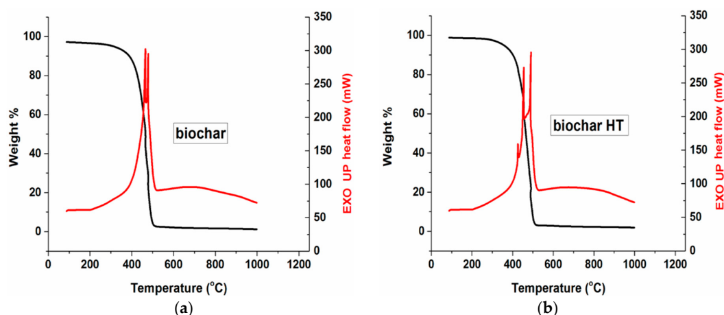
Figure 2. TGA-DSC curves of (a) biochar and (b) biochar HT.
