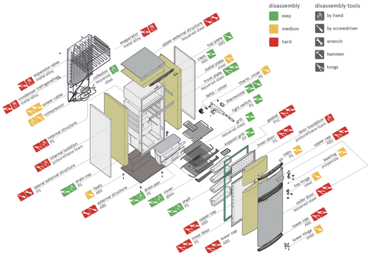
Figure 2. An example of a product (a refrigerator) broken-down into its individual components.
