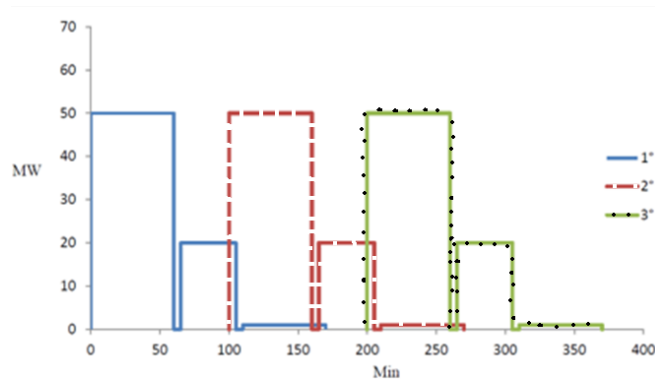
Fig. 2. Three cycles in series.
