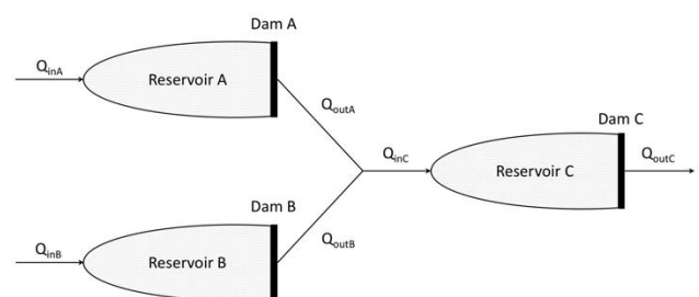
Fig.1: Tandem reservoir system model.
