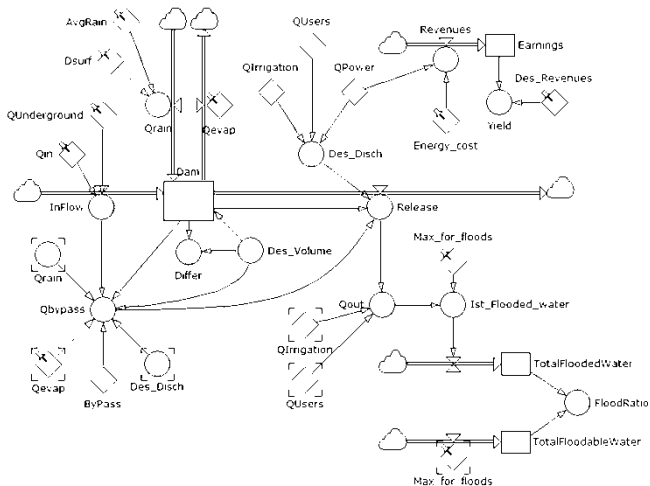
Fig.3: Dynamic model.
