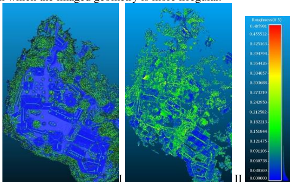
Figure 16. Roughness analysis of the PhotScan (I) and the VisualSfM (II) point clouds.
