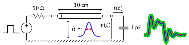
Fig. 1. Illustration of a stochastic transmission line problem: the deterministic excitation of a wire at random height produces a random response.
