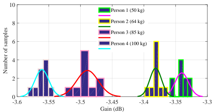
Fig. 9: Measurements distributions at f_c = 10 kHz.
