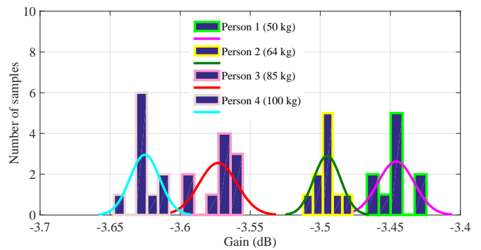
Fig. 10: Measurements distributions at f_c = 20 kHz.
