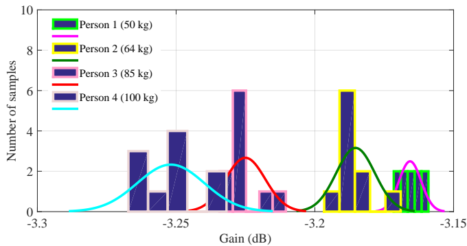
Fig. 8: Measurements distributions at f_c = 5 kHz.
