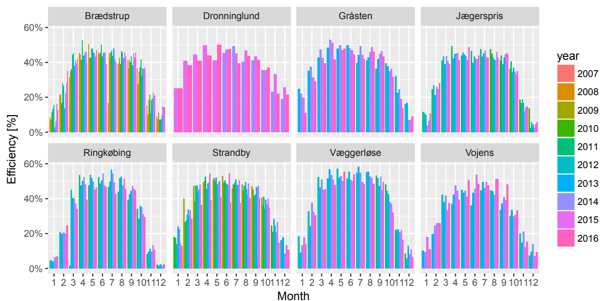
Fig. 5. Monthly conversion efficiency (selected systems)
