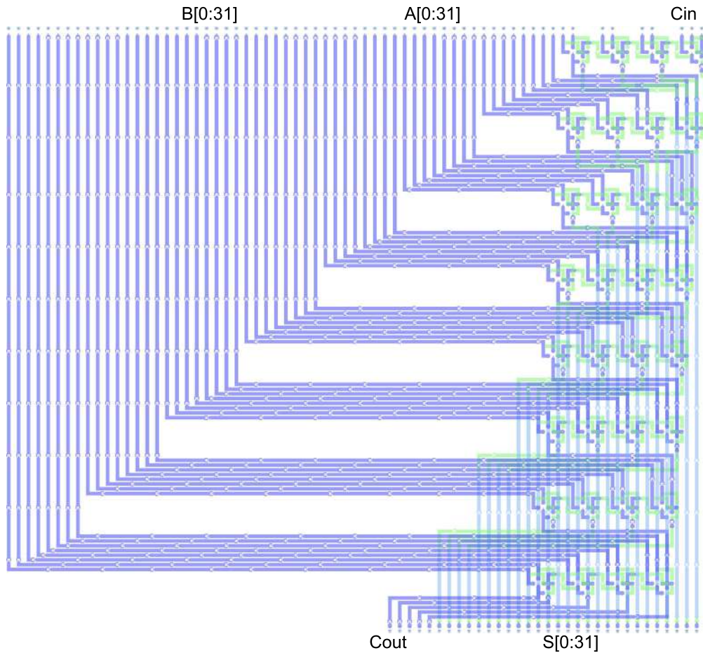
FIGURE 8. 3-D layout of the 32-bit Ripple Carry Adder.
