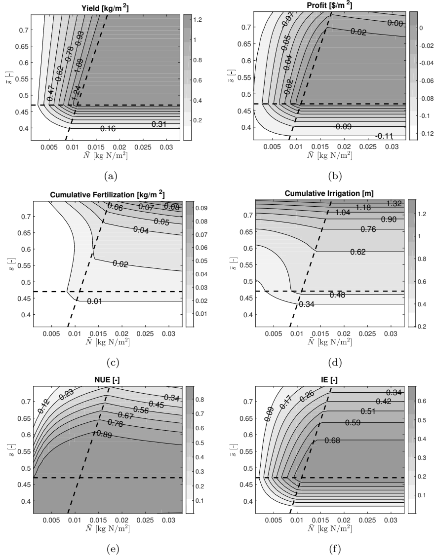
Figure 8: Response to the necessary rates of irrigation and fertilization to keep S and N at the designated constant values of (a) crop yield, (b) profit, (c) cumulative fertilization [kg/m 2 ], (d) cumulative irrigation [m], (e) Nitrogen use efficiency (NUE), the cumulative nitrogen uptake as a fraction of total fertilization, and (f) irrigation efficiency (IE), the cumulative transpiration as a fraction of the total irrigation. The horizontal dashed line represents the S^* threshold, while the diagonal dashed line is the \eta_c limit. All figures are for deterministic conditions (i.e., no stochastic forcing in the rainfall).
