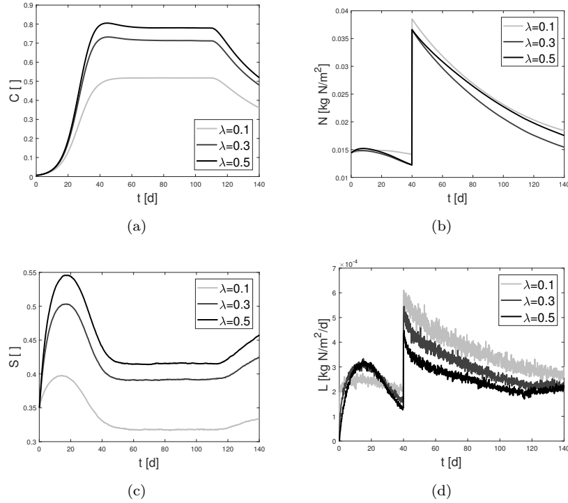
Figure 7: A comparison of the mean (a) canopy cover, (b) soil nitrogen, (c), soil moisture, and (d) leaching across different precipitation regimes for \lambda = 0.1 d -1 (light gray), \lambda = 0.3 d -1 (gray), \lambda = 0.5 d -1 (black), with \alpha altered to keep a constant mean rainfall rate of 4.5 mm/d for all figures. A typical fertilization treatment for corn has been applied, resulting in the observed jump in N .
