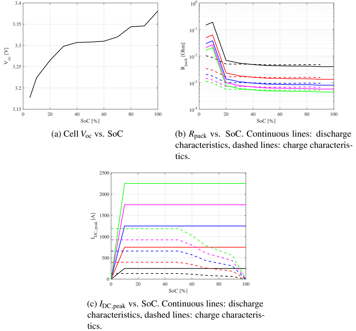
Fig. 4.1 Characteristics of the Li - Ion battery under consideration. (a) Cell open circuit voltage vs. SoC, (b) R_{pack} vs. SoC, (c) I_{DC,peak} vs. SoC. Black lines: Q_{nom} = 4.4Ah , red lines: Q_{nom} = 13.2Ah , blue lines: Q_{nom} = 22Ah , magenta lines: Q_{nom} = 30.8Ah , green lines: Q_{nom} = 39.6Ah . Data provided by the industrial partner of the project.
