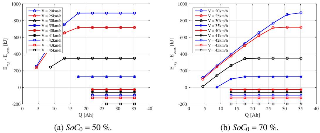
Fig. 4.12 Difference between recovered and consumed energy over an NEDC cycle as a function of the battery capacity for different maximum electric traction speeds considering SoC_0 = 50\% (a) and SoC_0 = 70\% (b).
