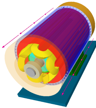
Fig. 3.32 Designed motor in Moor-CAD, 3D view.
