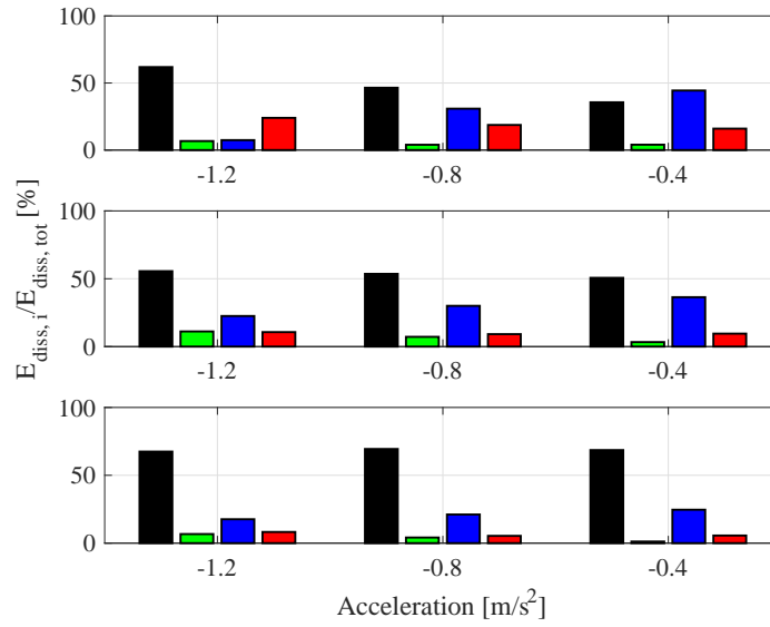
Fig. 2.5 Ratio between i^{th} and total dissipated energy vs. vehicle deceleration for different vehicle initial speeds. Top: 30 km/h, middle: 60 km/h, bottom: 100 km/h. Black bars: E_{diss,res} , green bars: E_{diss,pwt} , blue bars: E_{diss,ice} , red bars: E_{diss,bds} .
