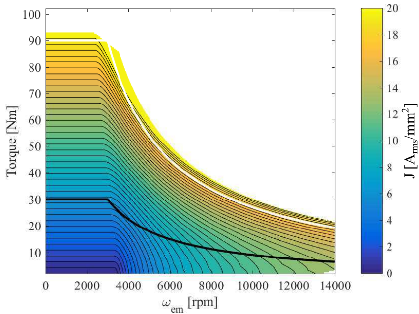
Fig. 3.24 Contour plot of current density [A_{\text{rms}}/\text{mm}^2] as a function of the electric motor torque and speed together with peak torque - speed curve (white) and continuous one (black).
