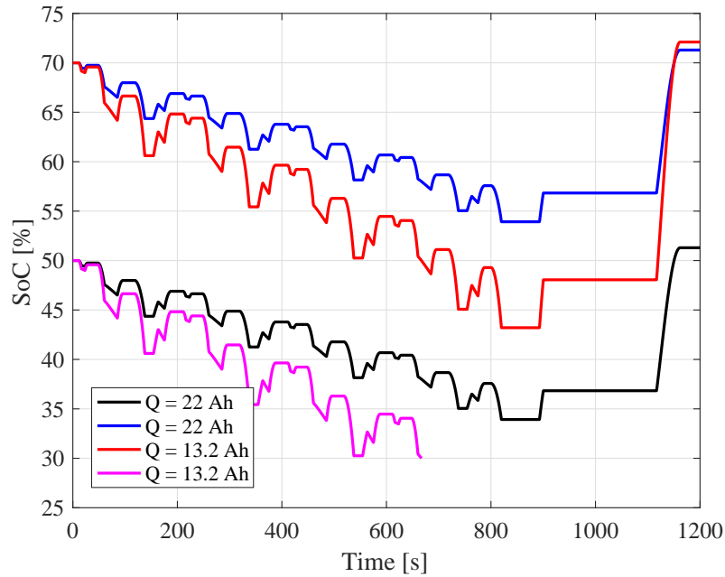
Fig. 4.14 Battery capacity influence on the battery state of charge along a NEDC cycle considering the same consumed energy for all the simulations ( V_{max,PE} = 39 km/h).
