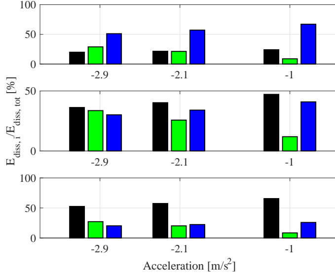
Fig. 2.8 Ratio between i^{th} and total dissipated energy vs. vehicle deceleration for different vehicle initial speeds. Top: 20 km/h, middle: 60 km/h, bottom: 100 km/h. Black bars: E_{diss,res} , green bars: E_{diss,pwt,r} , blue bars: E_{ICE} .
