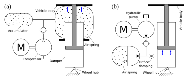
Figure 3. (a) Pneumatic and (b) Hydro-pneumatic height adjustment system schematics.
