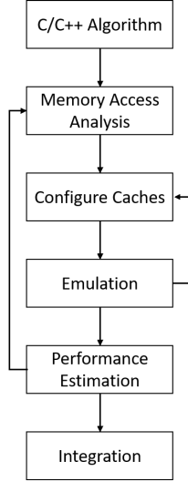
Fig. 4. Design flow with caches
