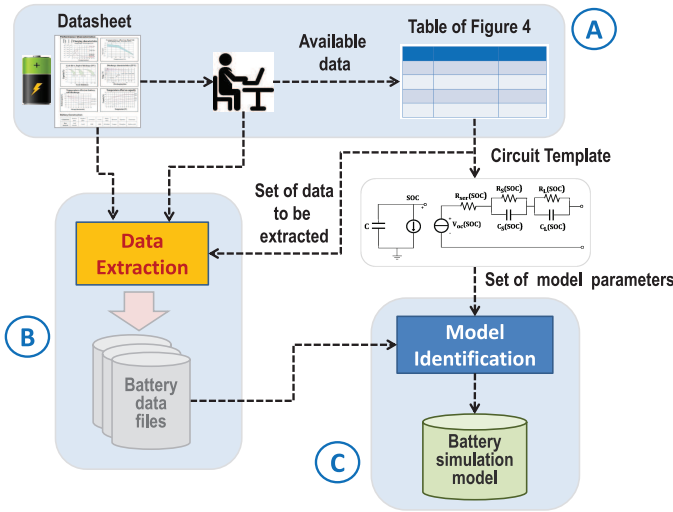
Fig. 3. Methodology flow
