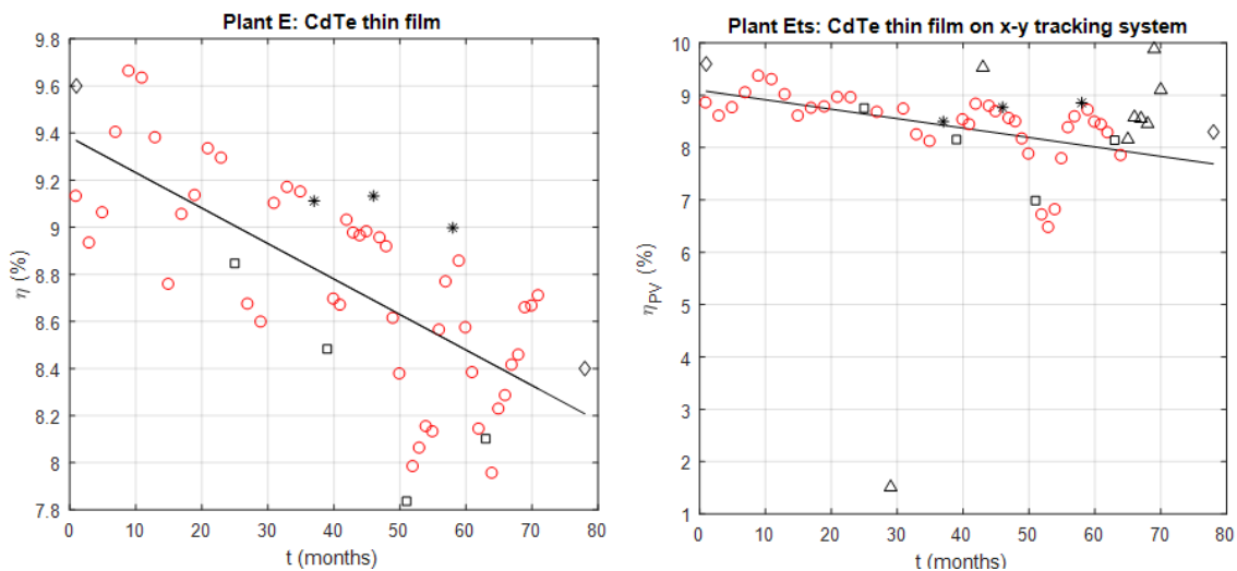
Figure 4. Estimated efficiency of the plants based on CdTe PV modules: E in fixed installation, E_{ts} on x-y tracking system.
