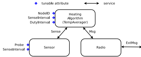
Figure 38.8 Module structure of example node-level WSN application.
