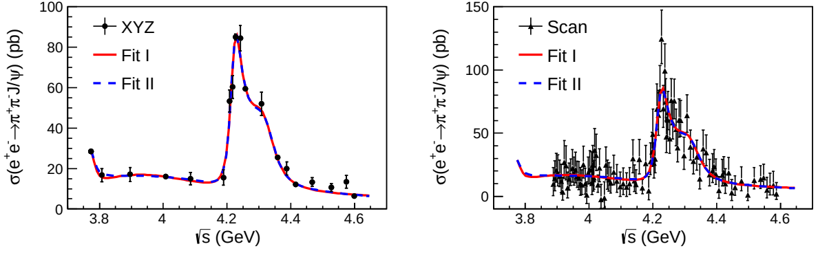
FIG. 1: Measured cross section \sigma(e^+e^- \rightarrow \pi^+\pi^- J/\psi) and simultaneous fit to the “XYZ data” (left) and “Scan data” (right) with the coherent sum of three Breit-Wigner functions (red solid curves) and the coherent sum of an exponential continuum and two Breit-Wigner functions (blue dashed curves). Dots with error bars are data.
