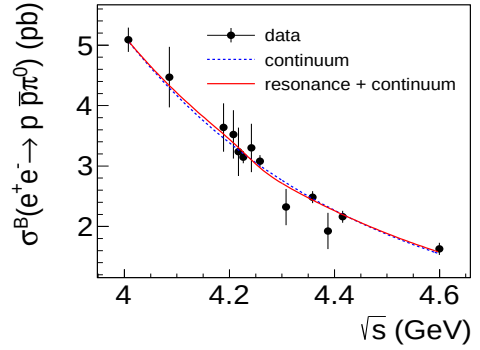
Figure 2: Fit to \sigma(e^+e^- \rightarrow p\bar{p}\pi^0) with resonance and continuum (solid line), or only continuum term (dashed line). Dots with error bars are the measured Born cross sections. The uncertainties are statistical only.
