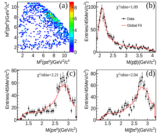
Figure 1: (a) Dalitz plot for the selected e^+e^- \rightarrow p\bar{p}\pi^0 candidates of data and invariant mass spectra of (b) p\bar{p} , (c) p\pi^0 and (d) \bar{p}\pi^0 at \sqrt{s} = 4.258 \text{ GeV} . In (b), (c) and (d), the points with error bars show data and the red histograms show MC projections of partial wave analysis fit described in the text.
