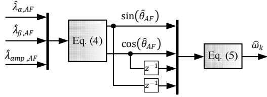
Fig. 6. Rotor position and speed observer.
