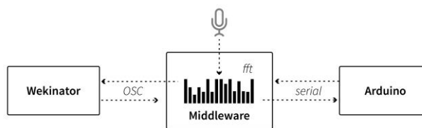
Figure 12 | Software architecture.
