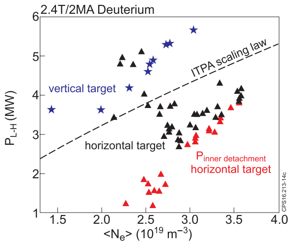
Figure 15. L–H threshold power at 2.4 T/2 MA for two magnetic configuration (vertical and horizontal target blue stars and black triangles) and power threshold for detachment of the inner divertor leg in the horizontal target configuration (red triangles) [117]. The dashed line correspond to the ITPA scaling [112].
