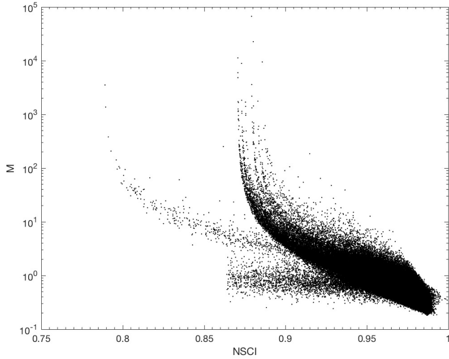
Figure 5: Truss structure: plot of the values of M with respect to the corresponding NSCI.
