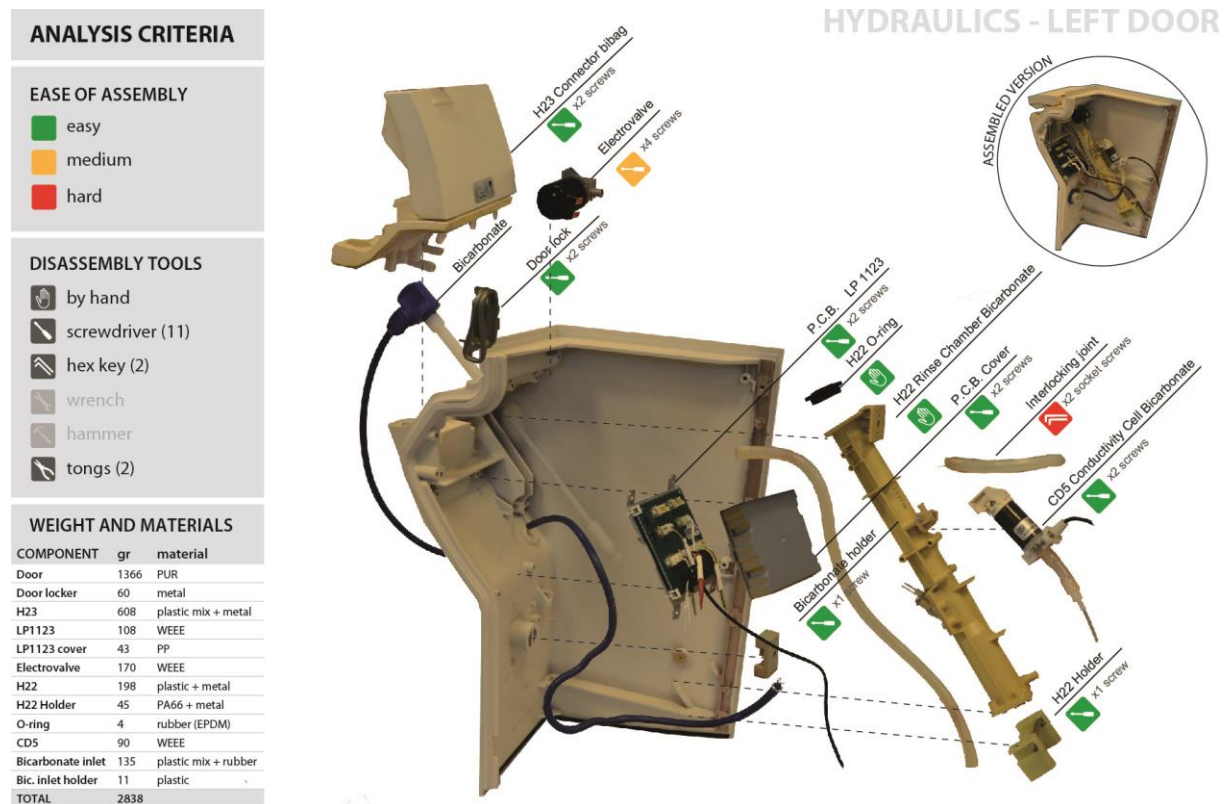
Figure 1. Example of Disassembly Analysis. The disassembly of a hydraulics macro-component is showed through a photographic exploded view. The tools needed to disassembly are visualized through icons, while the ease of assembly is indicated by means of a colour coding. The materials and weights of different components are summed up in a table.
