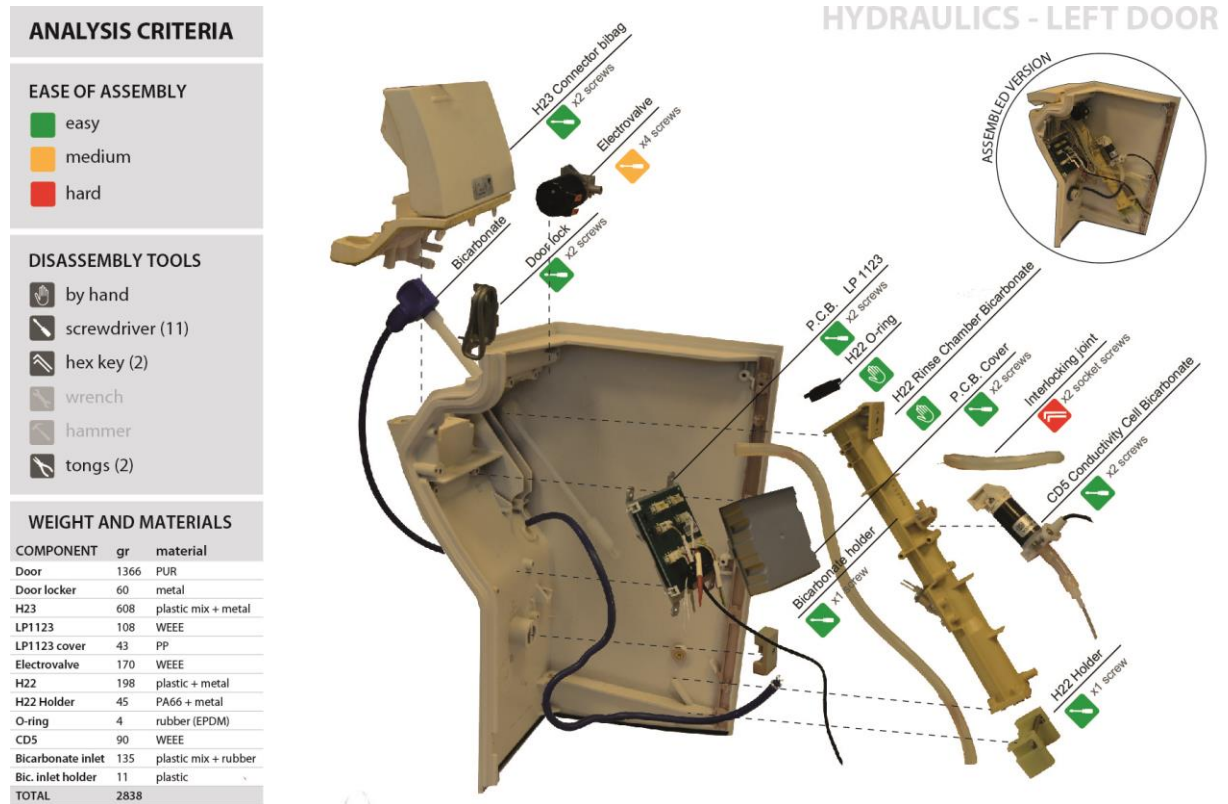
Figure 1. Example of Disassembly Analysis. The disassembly of a hydraulics macro-component is shown through a photographic exploded view. The tools needed to disassembly are visualized through icons, while the ease of assembly is indicated by means of a colour coding. The materials and weights of different components are summed up in a table.
