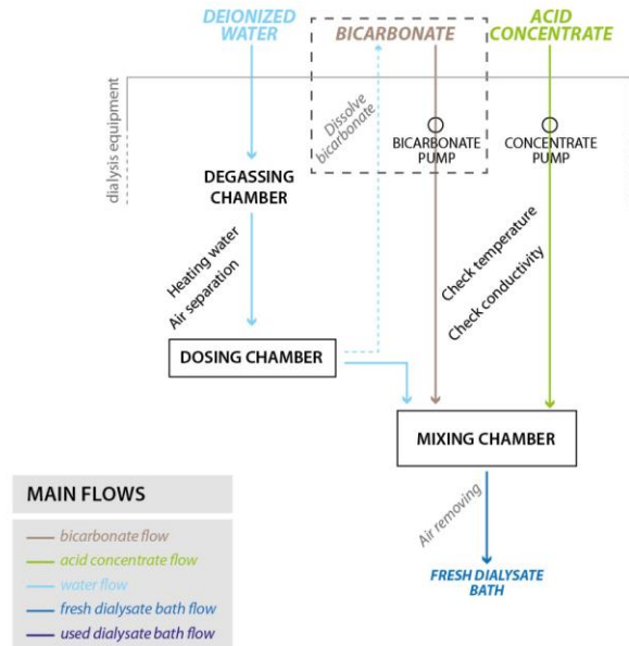
Figure 3. Example of general scheme (on the left) and essential scheme (on the right). The essential scheme brings together all the hydraulics macro-components that mix different material flows to obtain the fresh dialysate bath.
