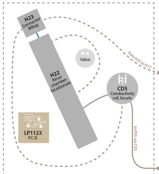
Figure 3. Example of general scheme (on the left) and essential scheme (on the right). The essential scheme brings together all the hydraulics macro-components that mix different material flows to obtain the fresh dialysate bath.
