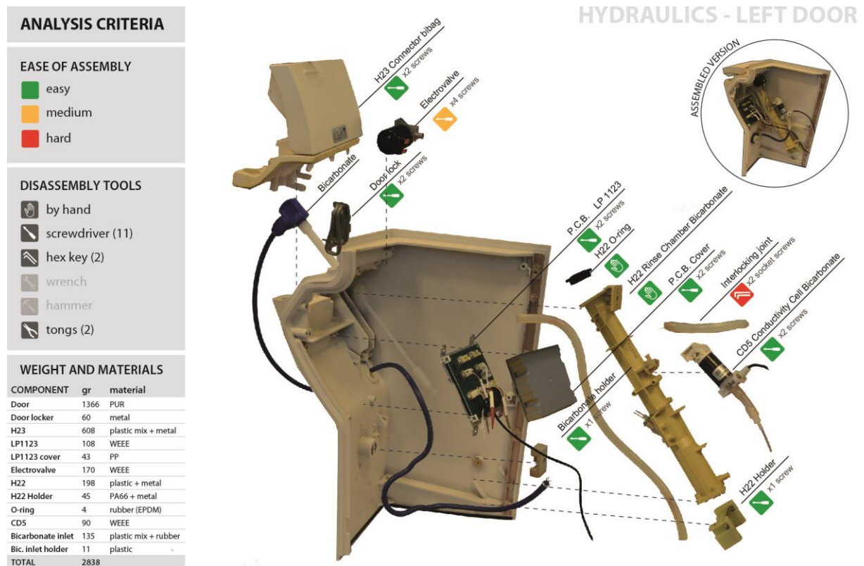
Figure 1. Example of Disassembly Analysis. The disassembly of a hydraulics macro-component is shown through a photographic exploded view. The tools needed to disassemble are visualized through icons, while the ease of assembly is indicated by means of a colour coding. The materials and weights of different components are summed up in a table.
