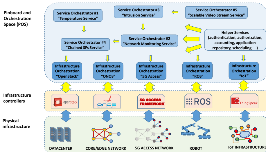
Fig. 1. 5G-OP architecture.
