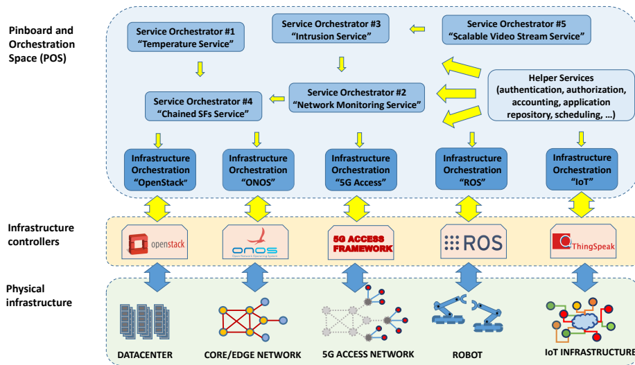
Fig. 1. 5G-OP architecture.
