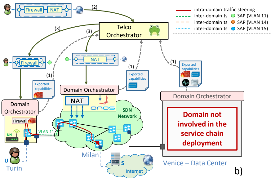
Fig. 4. Validation scenario: (a) service chain split across three domains; (b) service chain deployed in two domains.
