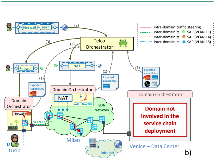
Fig. 4. Validation scenario: (a) service chain split across three domains; (b) service chain deployed in two domains.
