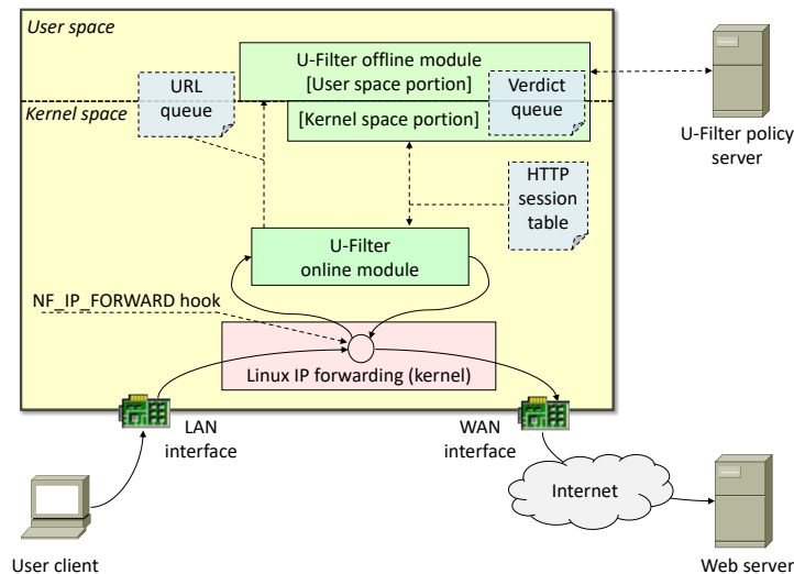
Figure 2: U-Filter architecture.
