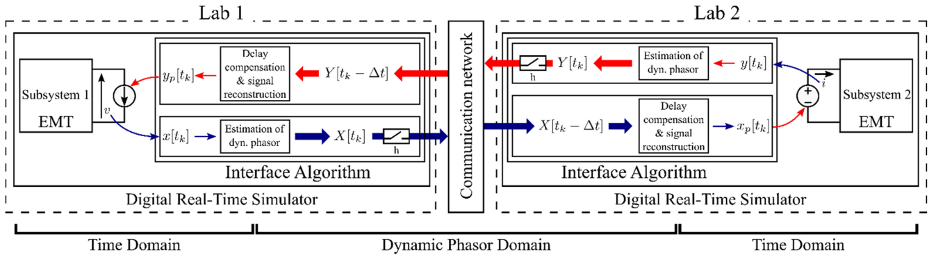
Fig. 4 Co-simulation IA
