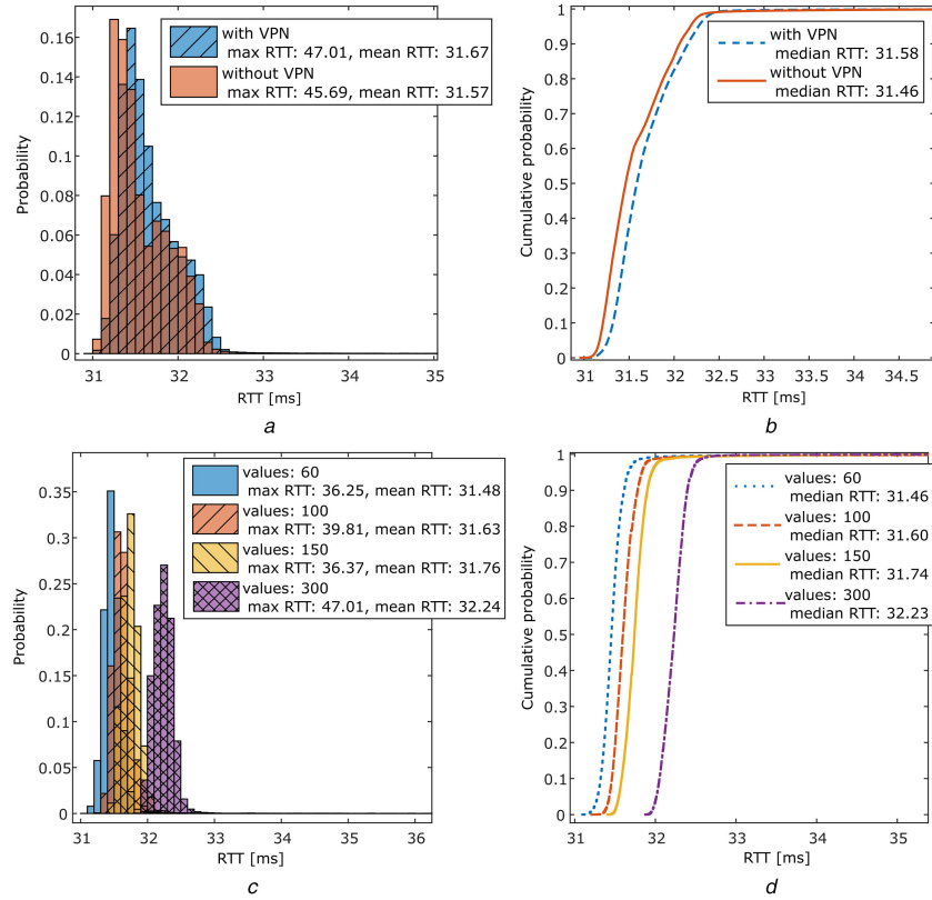
Fig. 3 RTT results of loopback communication tests between two laboratories for data exchange of UDP packets
