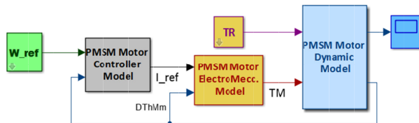
Fig. 2: Block diagram of the EMA numerical model
