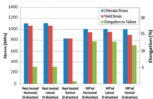
Figure 14. Tensile properties of DEDed Ti-6Al-4V in different building orientations after heat treatment and HIP process (reproduced with permission from [18] Copyright Elsevier, 2015).
